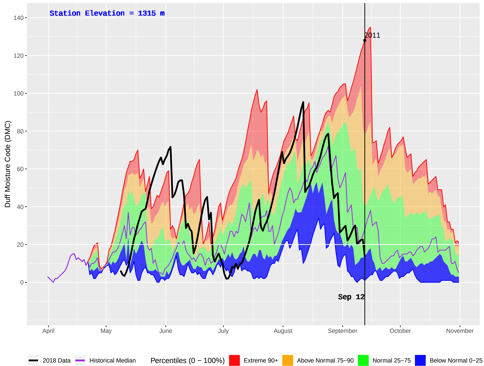
MAYSON (1082) : Historical (2010–2016) and Current (2018) Daily Duff Moisture Code (DMC)
