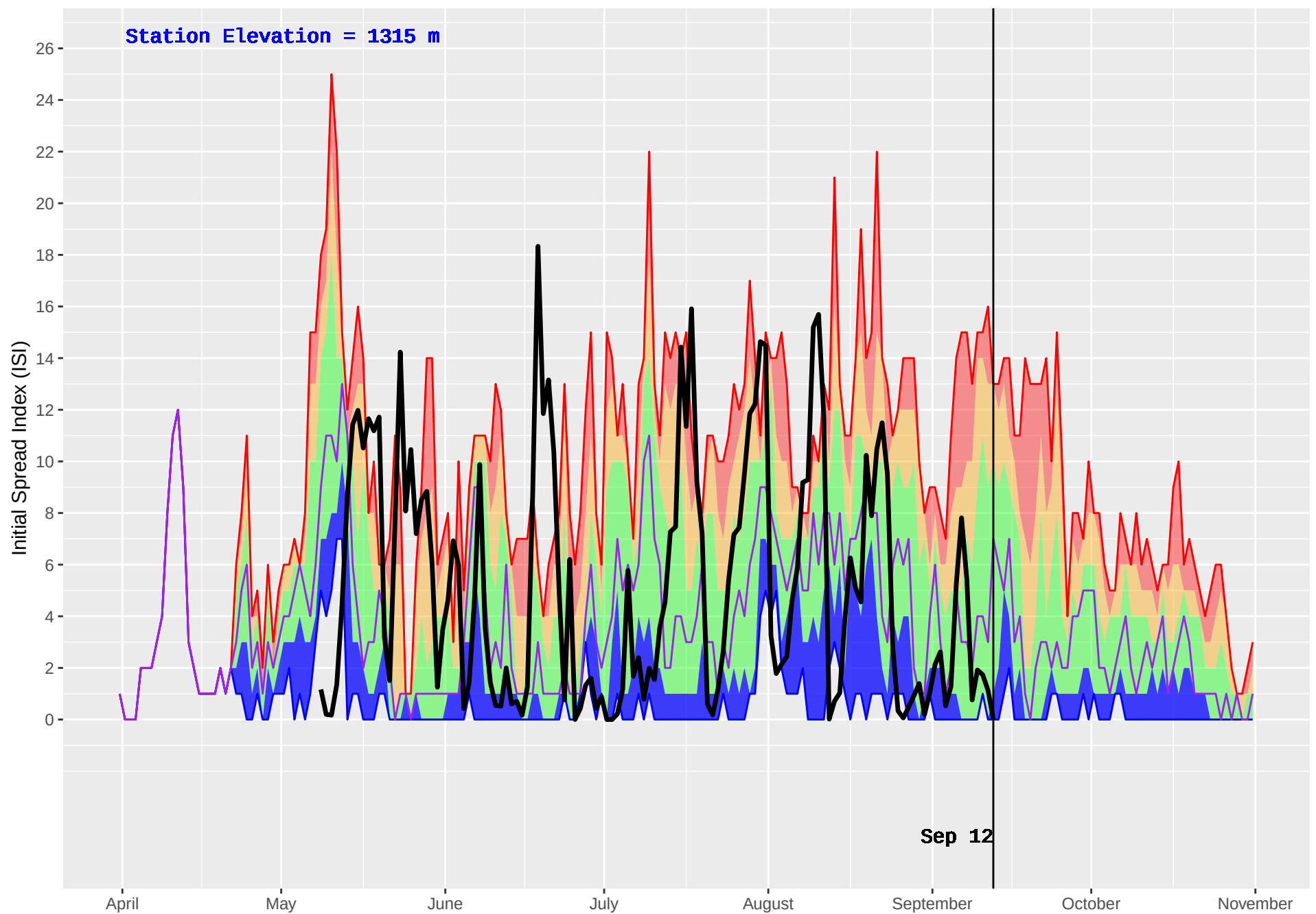
MAYSON (1082) : Historical (2010–2016) and Current (2018) Daily Initial Spread Index (ISI)
